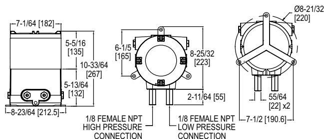
AT-102PA-A3000, shown with VS0 port/valve configuration
