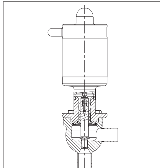
Fig. 3: Type 3347/3379 Control Valve with welding ends Version with bar stock body with flanged-on bonnet
