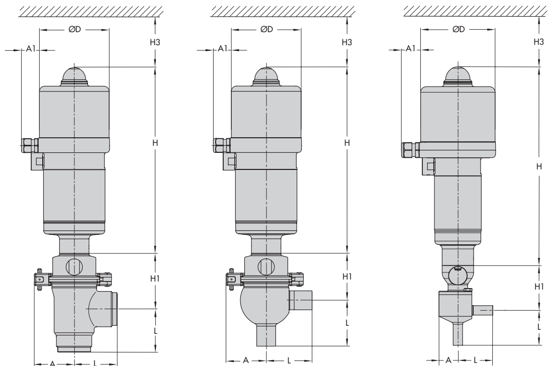
Type 3347/3379/3724 Control Valve with welding ends Version with cast body
