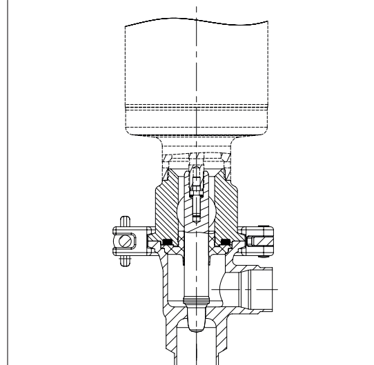
Fig. 4: Type 3347/3379 Control Valve with welding ends Version with cast body
