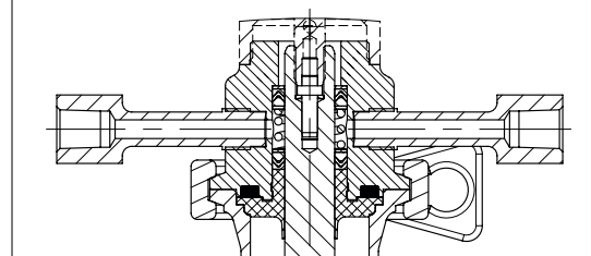
Fig. 5: Steam line connection
