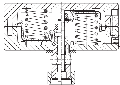
extends Actuator stem retracts
