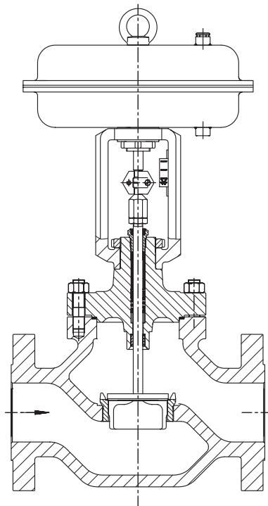
Fig. 2 · Type 3251-1 Control Valve with Type 3271 Pneumatic Actuator
